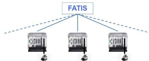
Figure 2: FATIS Scalability
