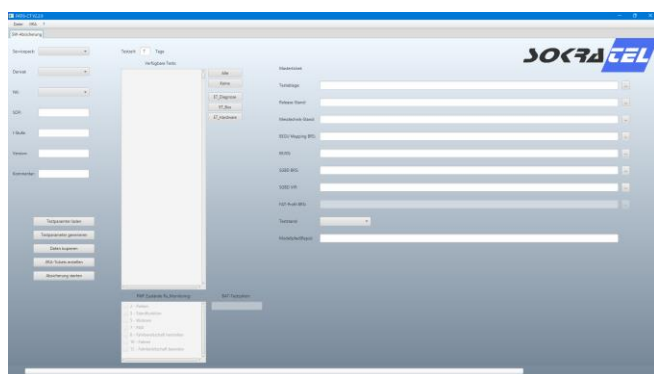
Figure 1: Screenshot FATIS-CT
